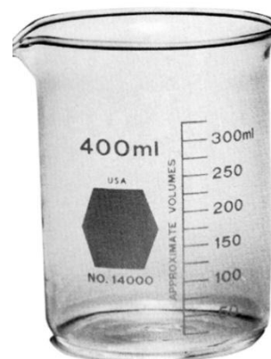
Beaker
