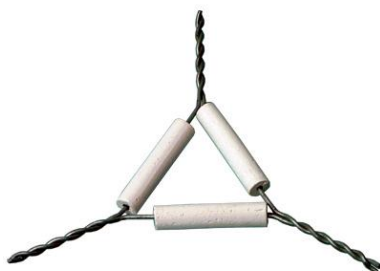
Clay triangle
