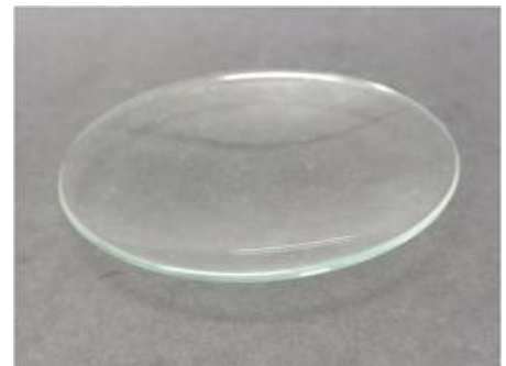
Watch glass
