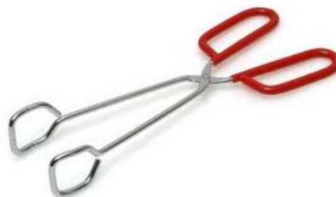
Tongs
