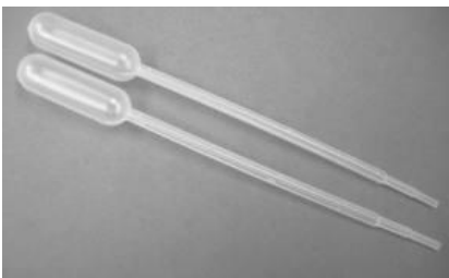
Plastic pipettes
